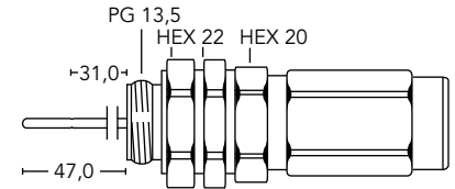
PG13,5mu-XX
