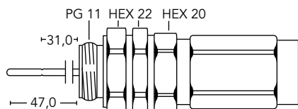
PG11mu-XX
